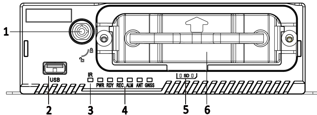
Front Panel
